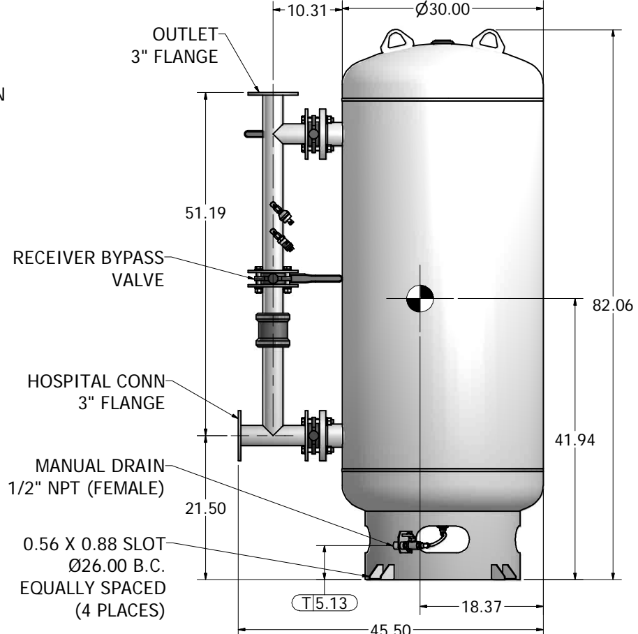
200 GAL VACUUM RECEIVER 3" FLANGED CONNECTIONS (SCALE 1:10)
