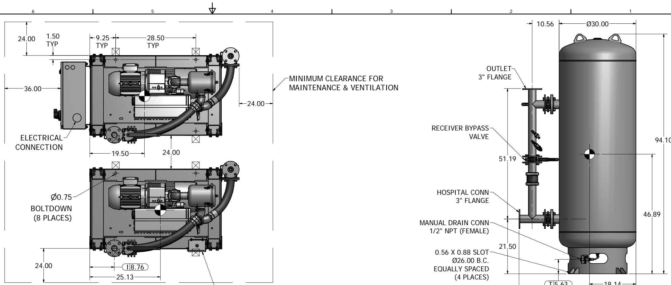
240 GAL VACUUM RECEIVER 3" FLANGED CONNECTIONS (NTS)
