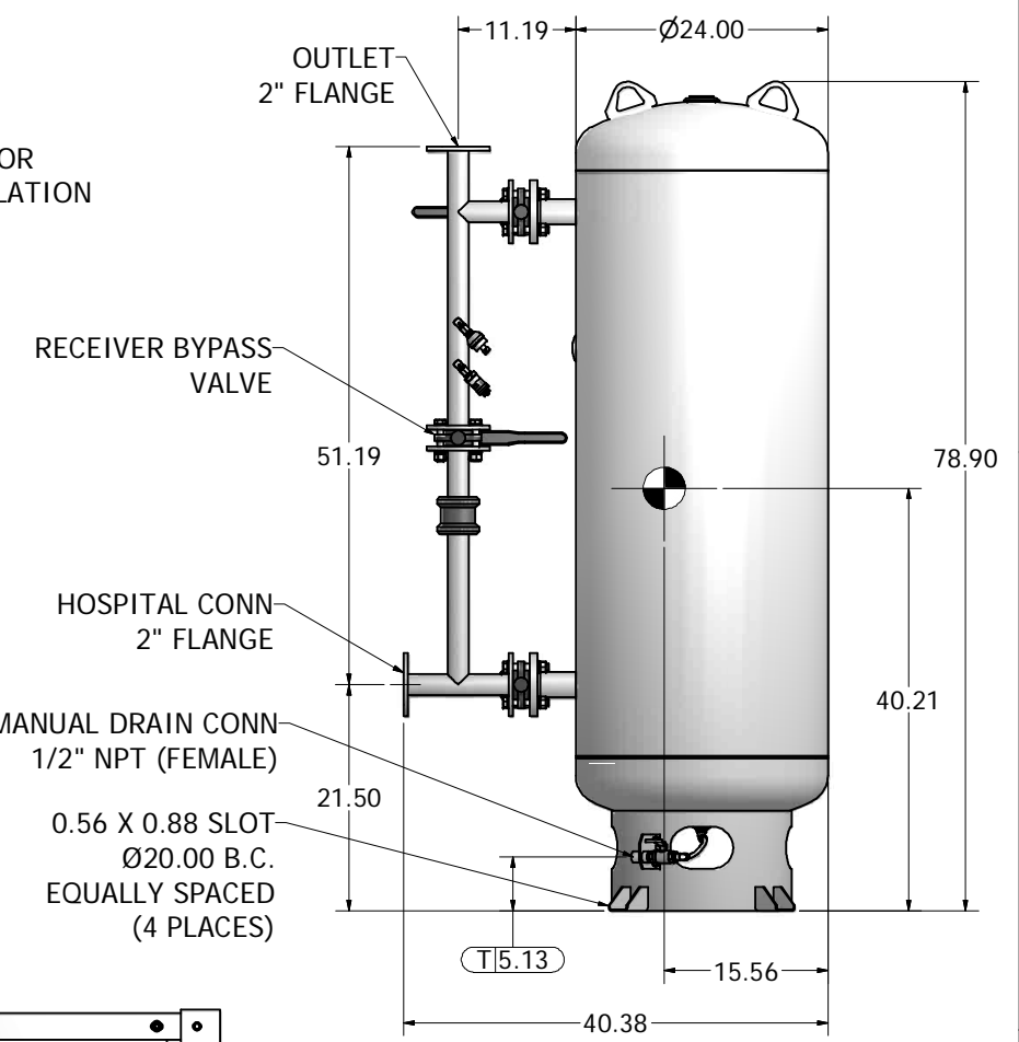
120 GAL VACUUM RECEIVER 2" FLANGED CONNECTIONS (SCALE 1:10)
