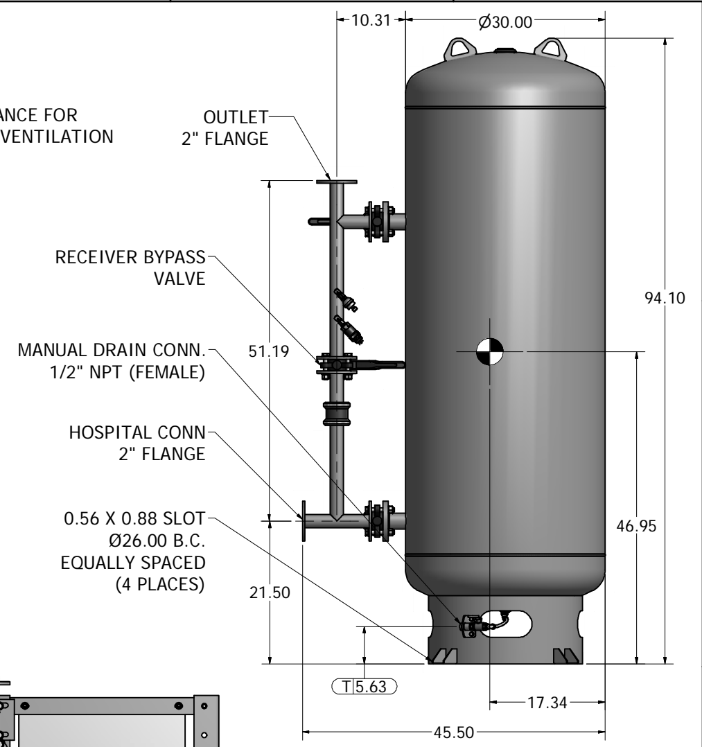
240 GAL VACUUM RECEIVER 2" FLANGED CONNECTIONS (SCALE 1:10)
