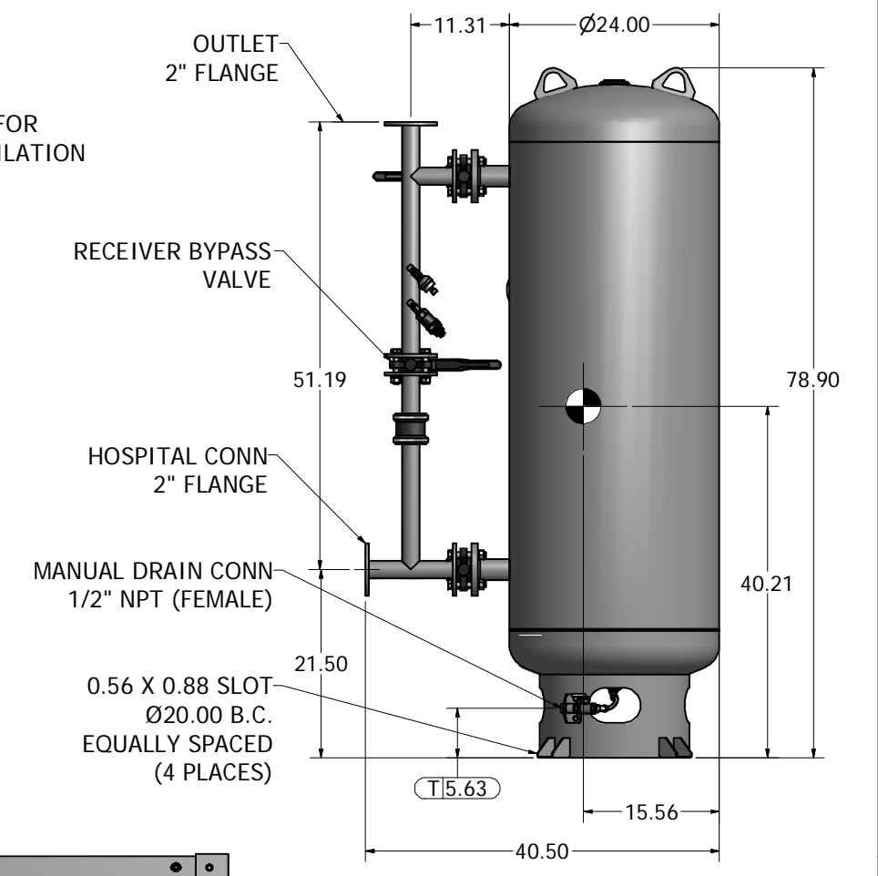
120 GAL VACUUM RECEIVER 2" FLANGED CONNECTIONS (SCALE 1:10)
