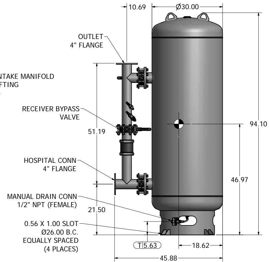
240 GAL VACUUM RECEIVER 4" FLANGED CONNECTIONS (SCALE 1:12)
