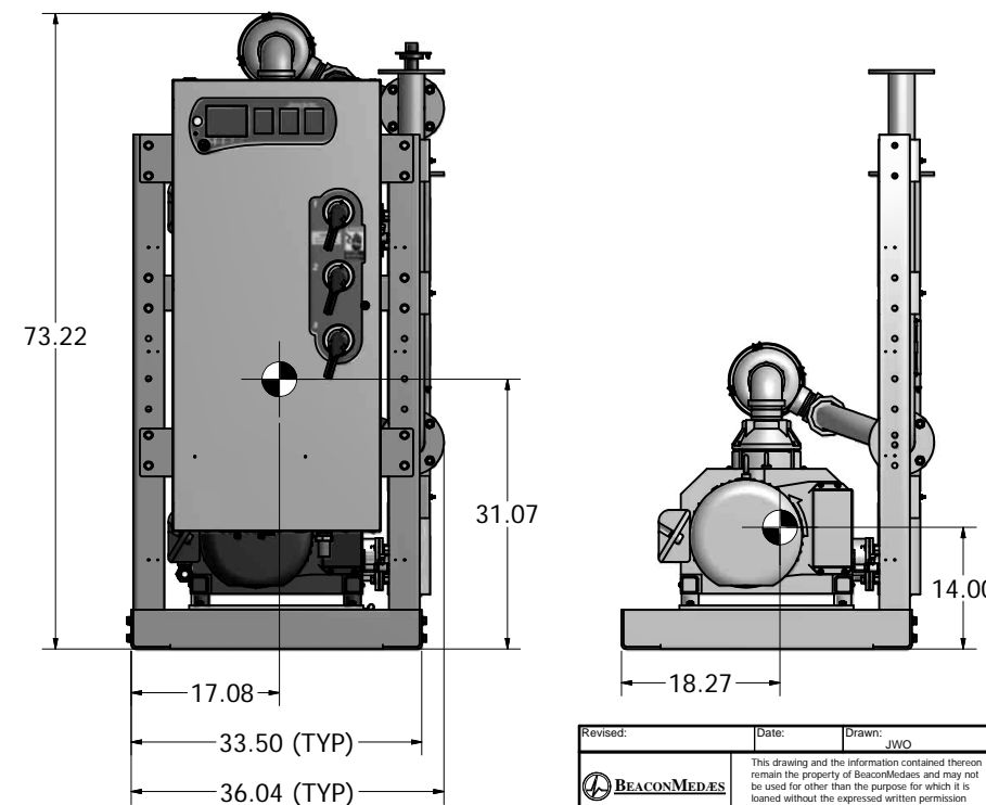
240 GAL VACUUM RECEIVER 4" FLANGED CONNECTIONS (SCALE 1:12)
