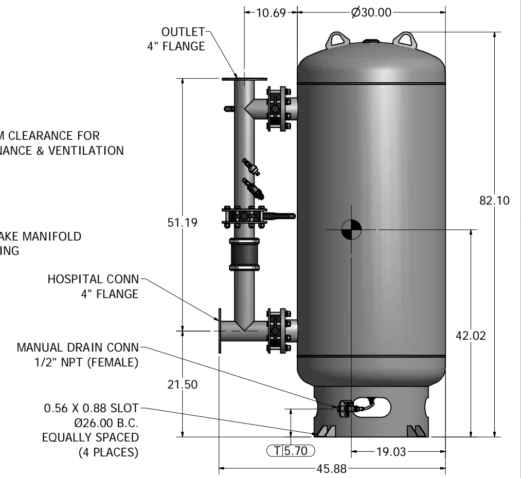
200 GAL VACUUM RECEIVER 4" FLANGED CONNECTIONS (SCALE 1:10)
