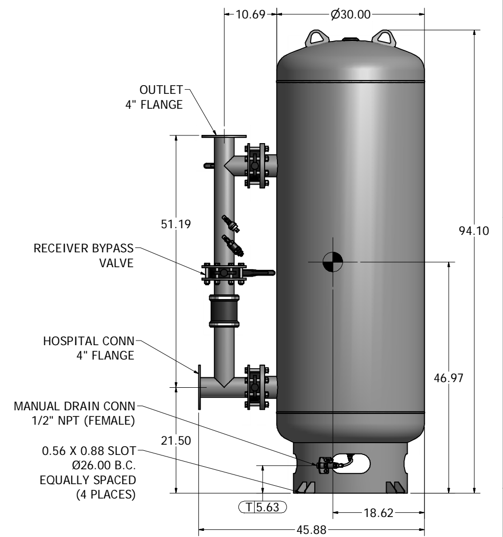
240 GAL VACUUM RECEIVER 4\"/>
