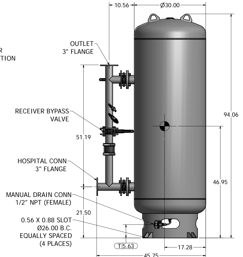
240 GAL VACUUM RECEIVER 3" FLANGED CONNECTIONS (SCALE 1:10)
