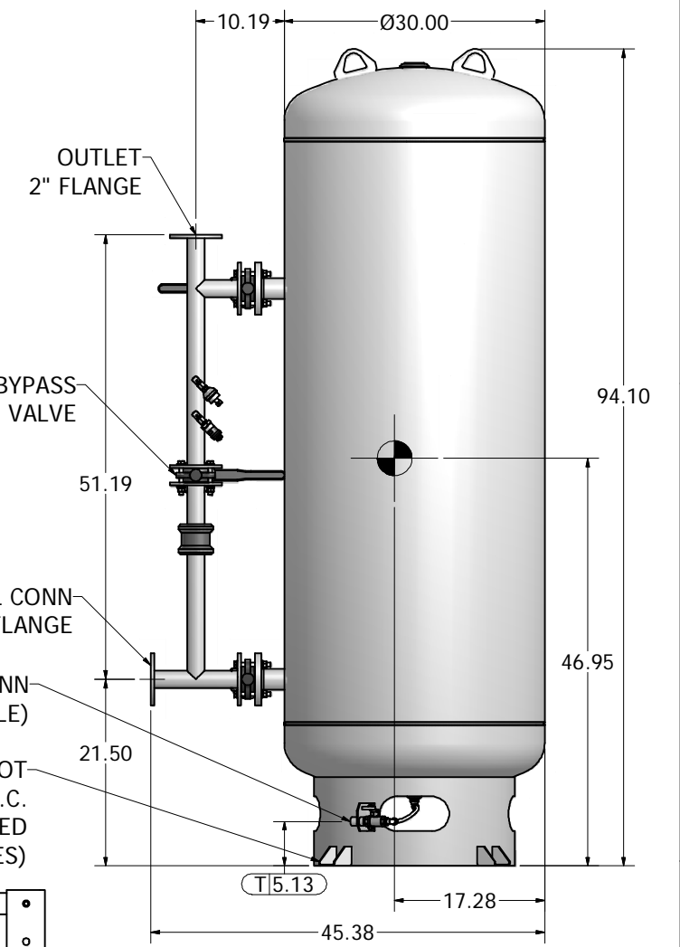
240 GAL VACUUM RECEIVER 2" FLANGED CONNECTIONS (SCALE 1:10)
