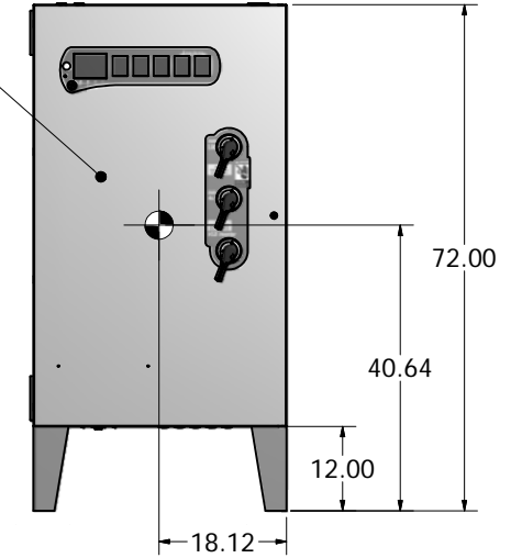
CONTROL PANEL
