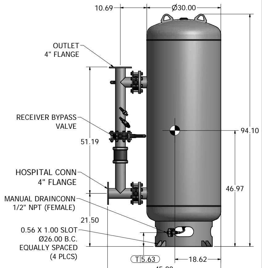
240 GAL VACUUM RECEIVER 4" FLANGED CONNECTIONS (SCALE 1:12)
