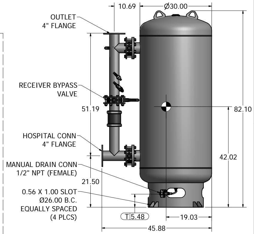
200 GAL VACUUM RECEIVER 4" FLANGED CONNECTIONS (SCALE 1:12)
