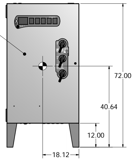
CONTROL PANEL
