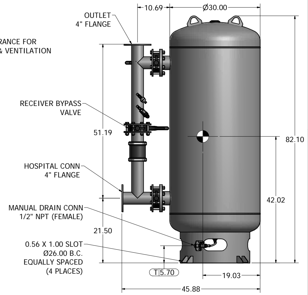
200 GAL VACUUM RECEIVER 4" FLANGED CONNECTIONS (SCALE 1:10)
