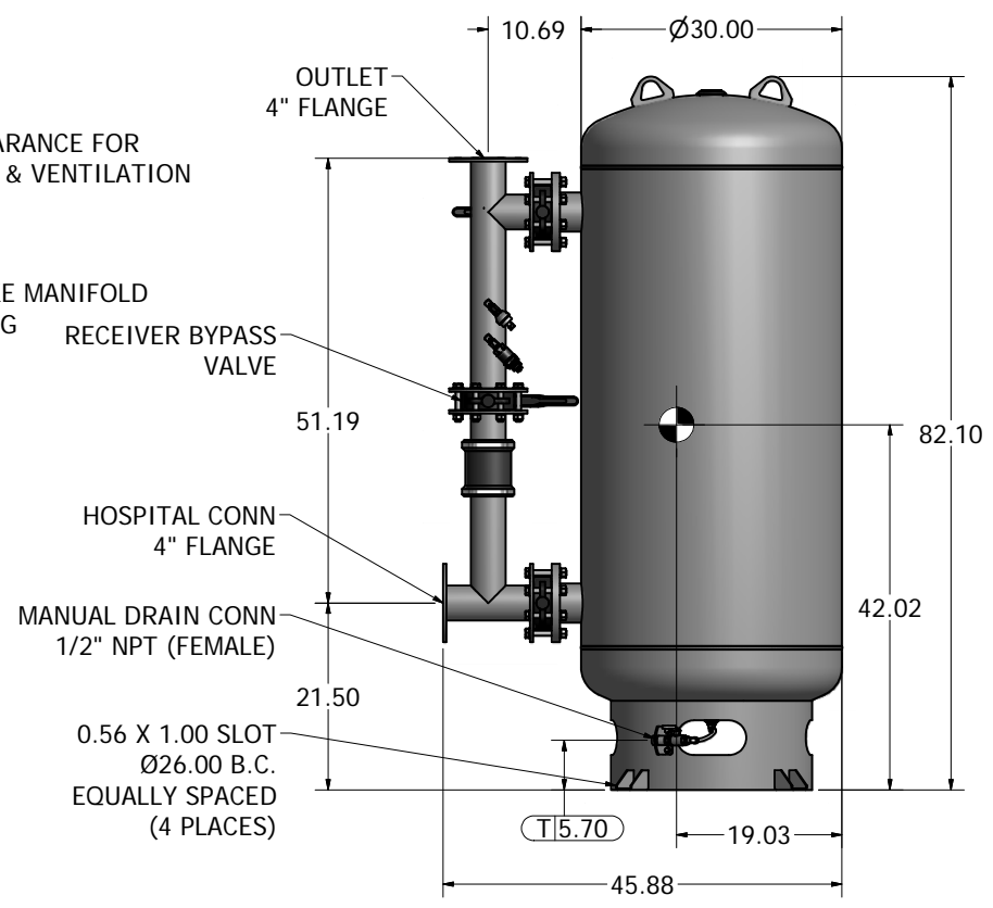
200 GAL VACUUM RECEIVER 4" FLANGED CONNECTIONS (SCALE 1:12)
