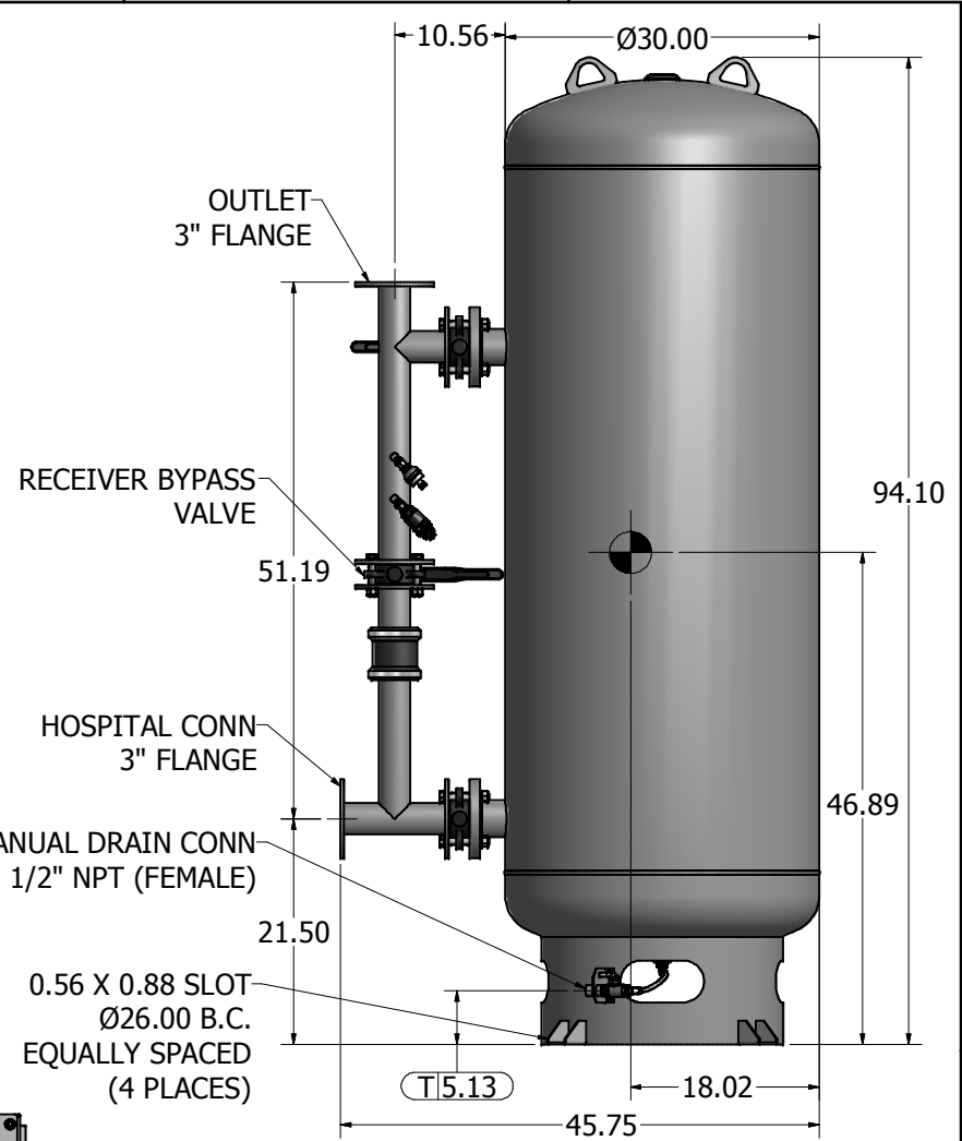
240 GAL VACUUM RECEIVER 3" FLANGED CONNECTIONS (SCALE 1:10)
