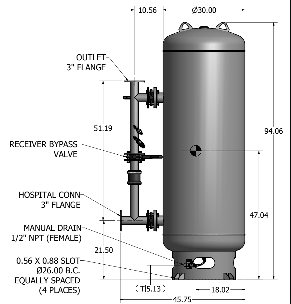
240 GAL VACUUM RECEIVER 3" FLANGED CONNECTIONS (SCALE 1:11)
